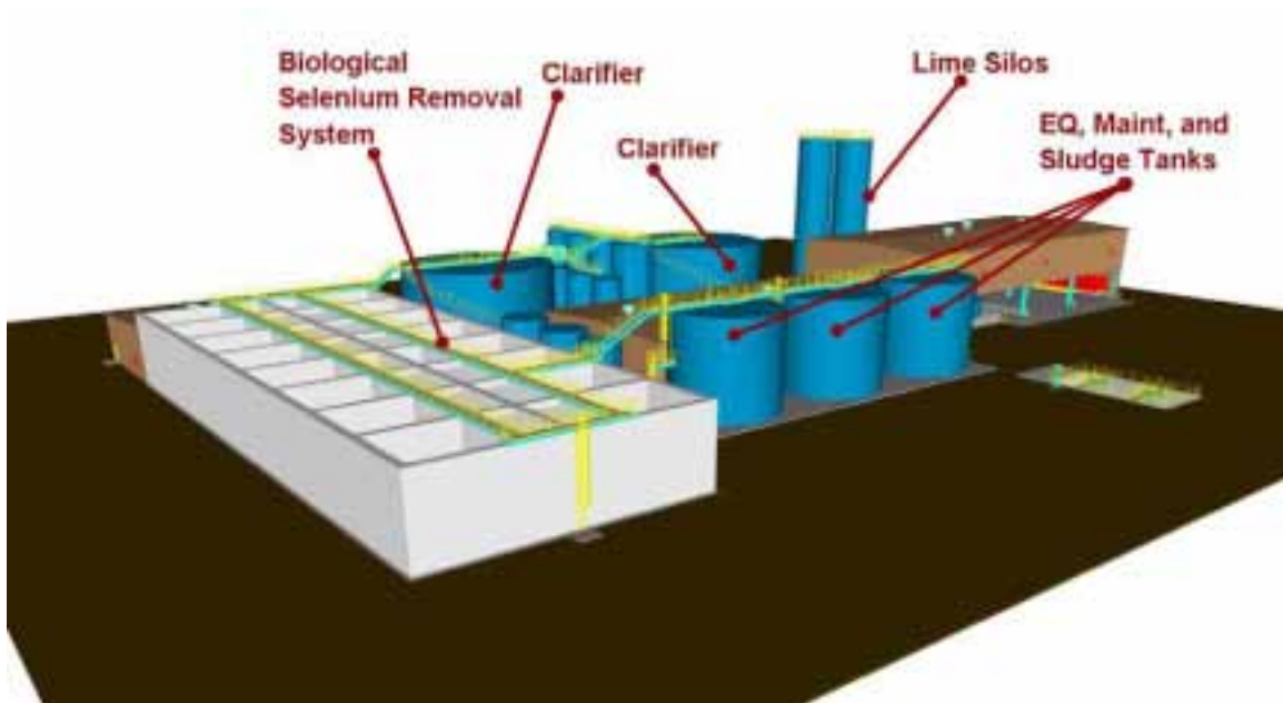
Figure 5: Artist Depiction of Belews Creek WWTS
