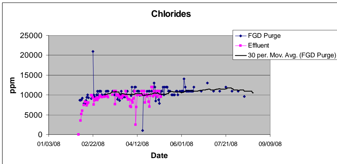
Figure 7: Chemical Characteristics for Belews Creek Operations
