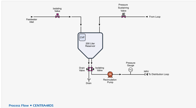
Process Flow ■ CENTRA-MDS
