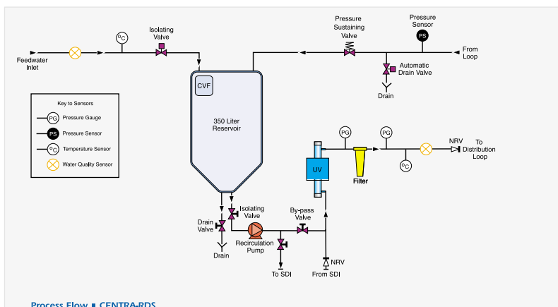
Process Flow ■ CENTRA-RDS
