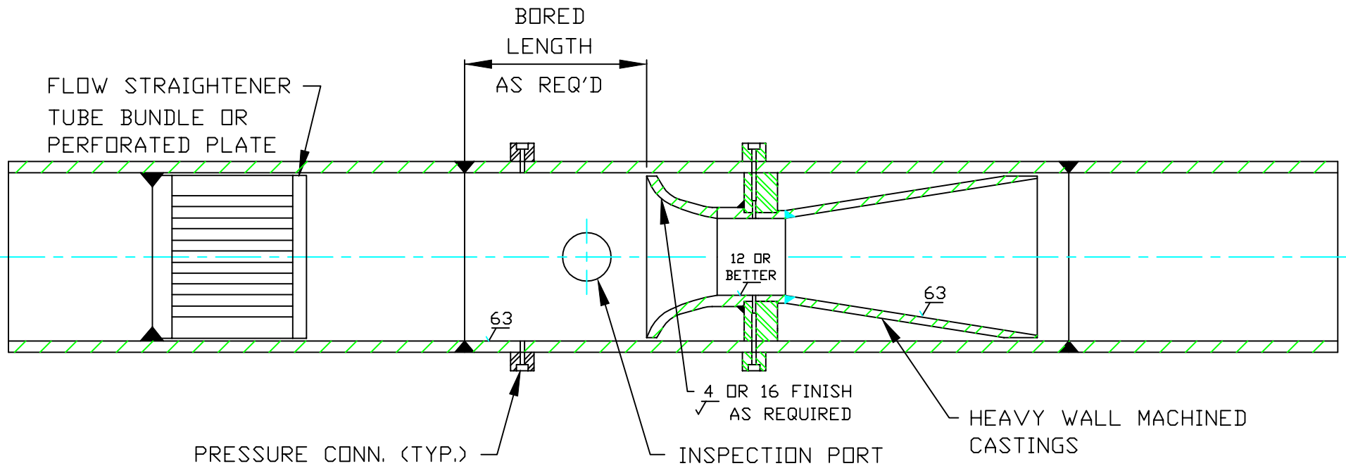
TYPICAL FEEDWATER FLOW METER (WELDED CONSTRUCTION).
