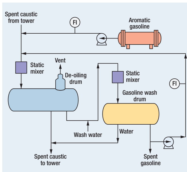
FIG. 3 Example gasoline washing step configuration.
