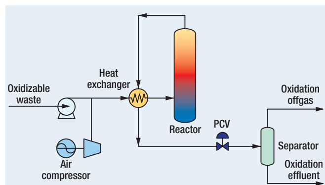
FIG. 1 Block flow diagram of WAO system.
